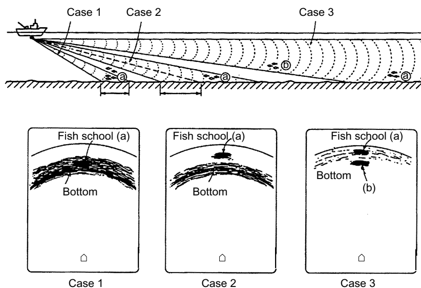
How to discriminate fish echoes from bottom
