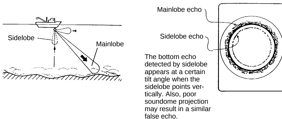
Sidelobe echo
